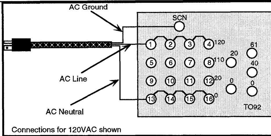
Figure 4-5. Transformer Wiring
